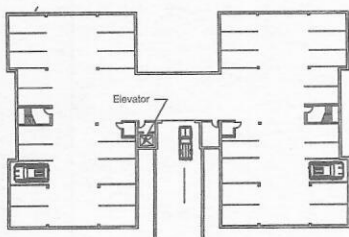
Parking Level
